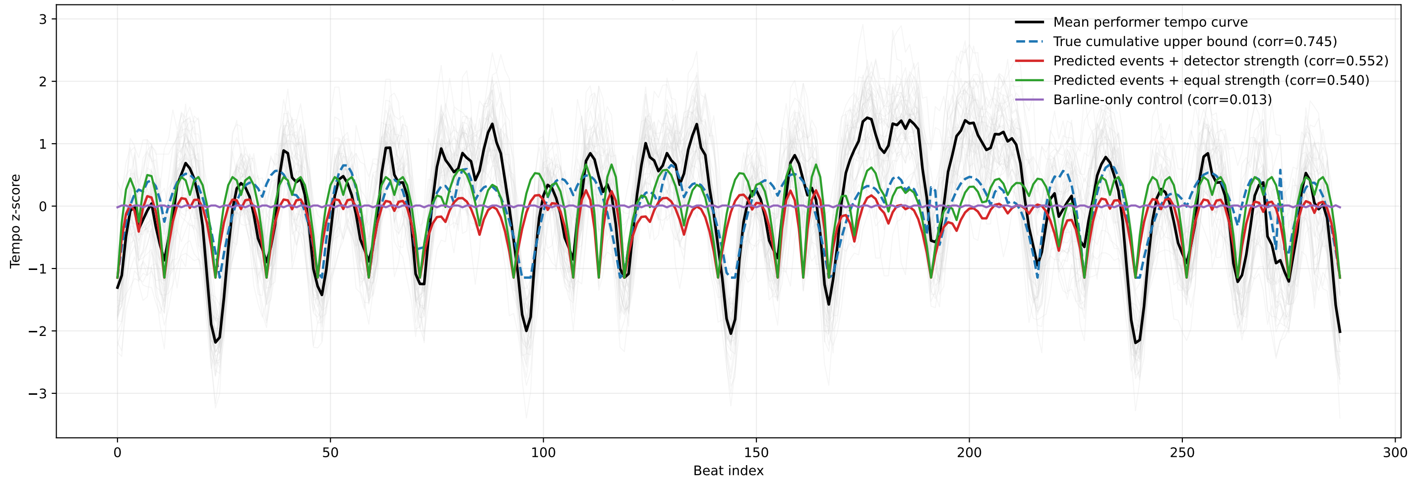
M06-2: tempo reconstruction controls
