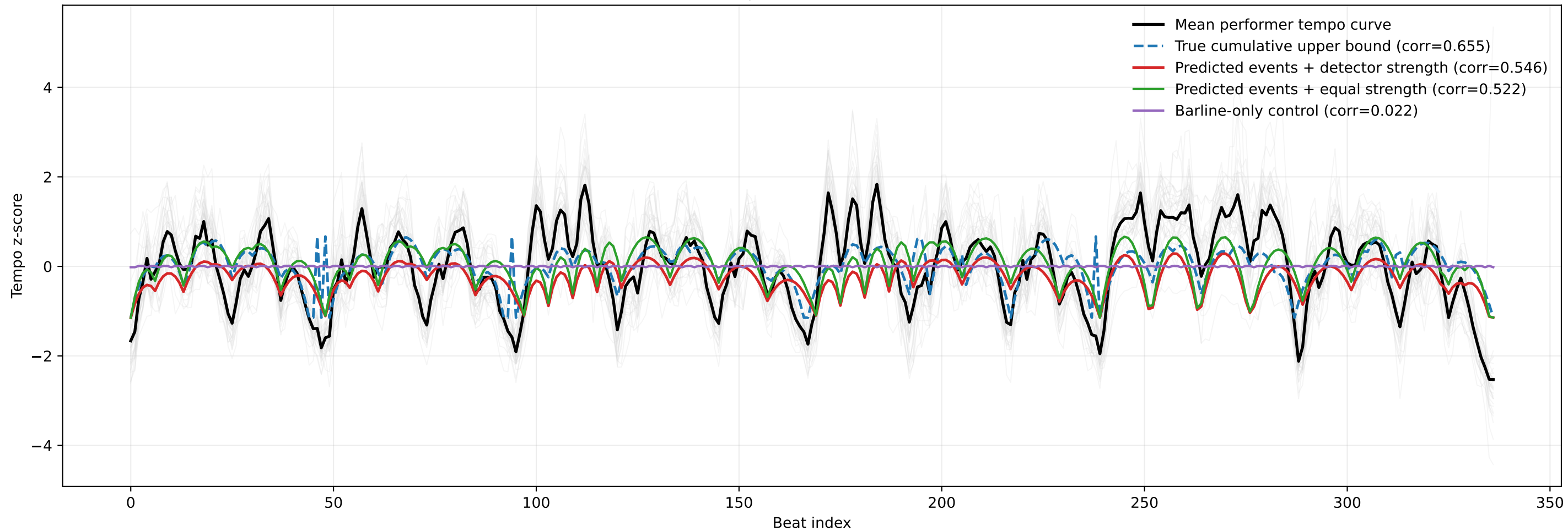
M06-1: tempo reconstruction controls
