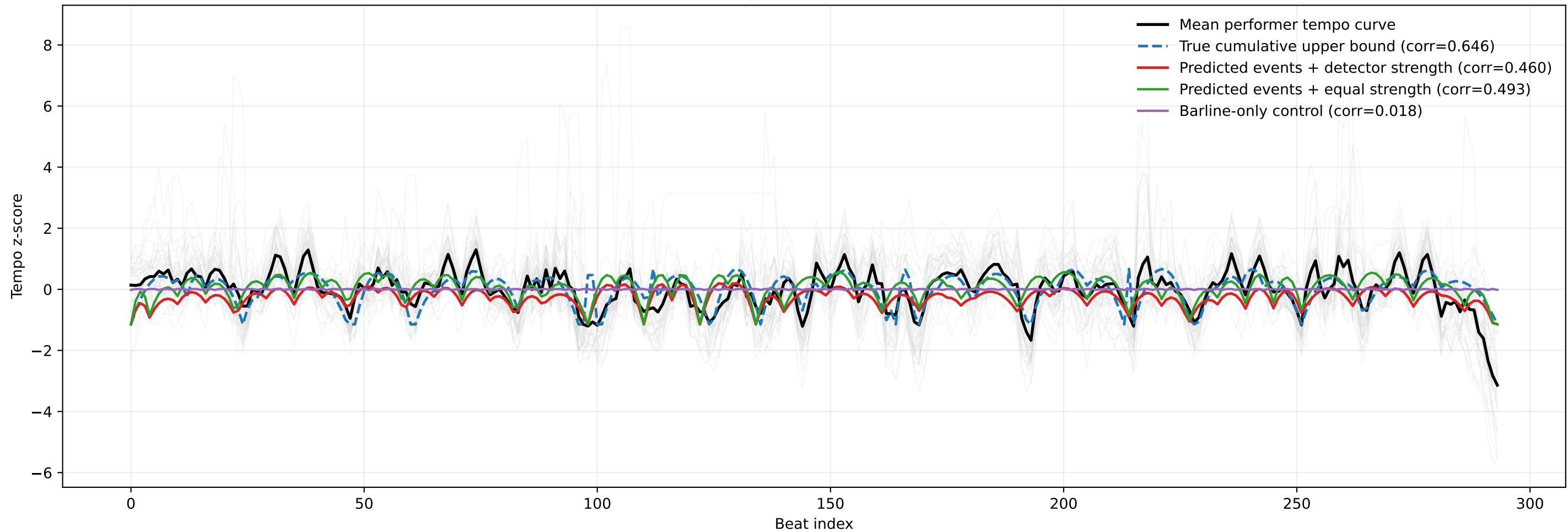
M06-3: tempo reconstruction controls
